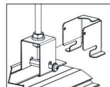
MS25 + MO24 Sports Hall Suspension Kit
