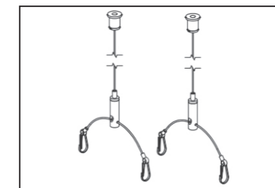
117.SUSK - SUSPENSION KIT FOR 117
